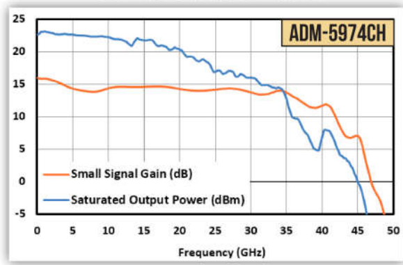
Gain & Output Power
