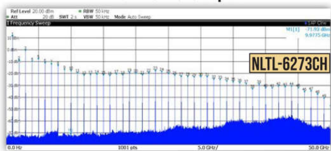
Harmonic Output
