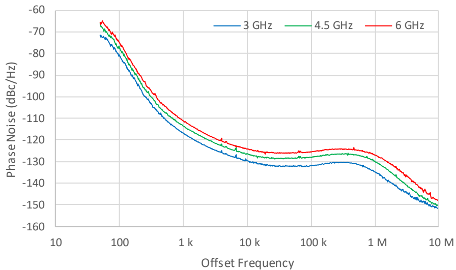
Measured phase noise
