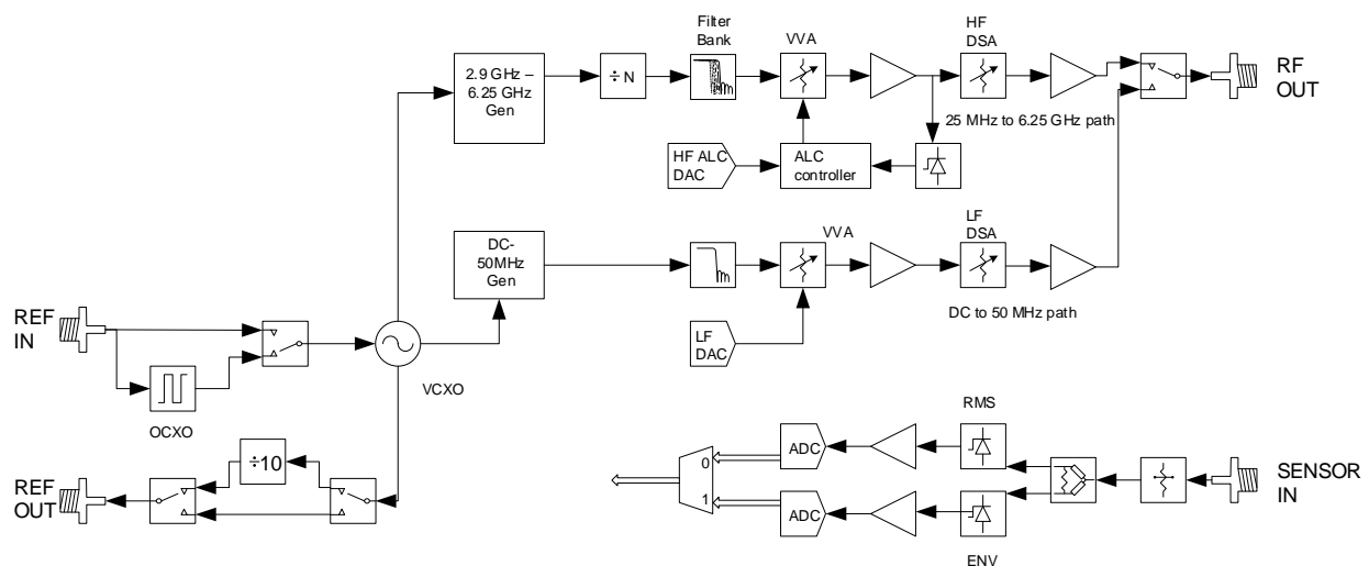
Figure 1. SC5507/8A Block Diagram
