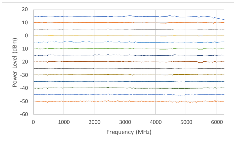
Measure Output power, ALC closed
