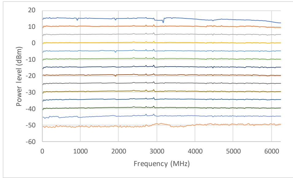
Measured output power, ALC opened
