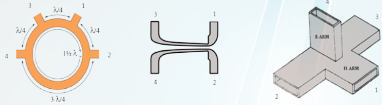
Fig. 10 Rat Race Coupler (left), asymmetric tandem coupler (center), and Waveguide Magic-T (right)
