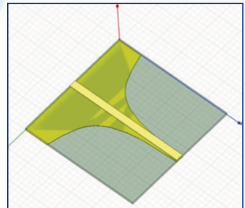
Fig. 6 Tapered microstrip balun
